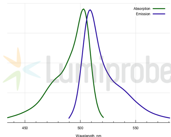
BDP FL absorption and emission spectra
