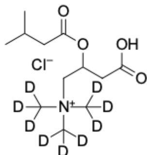
Structure of (C5) Isovaleryl-L-carnitine-(trimethyl-d9)
