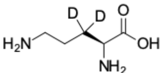
Structure of L-Ornithine-d2
