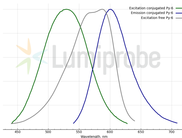
Excitation and emission spectra of Pyrylium-6 (Py-6)
