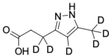
Structure of (SA) Succinylacetone-d6
