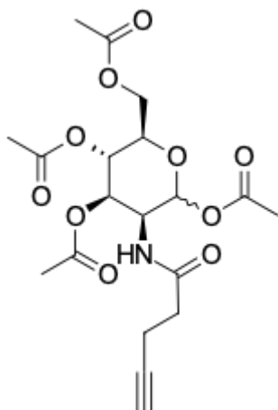
Structure of Ac4ManNAI (N-(4-pentynoyl)-mannosamine-tetraacylated)
